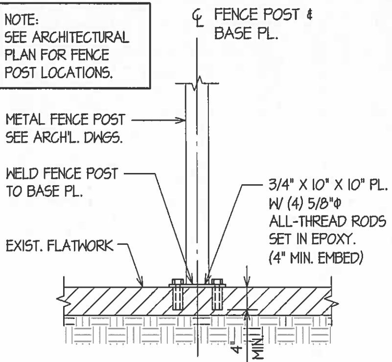
METAL FENCE POST BASE PLATE DETAIL AT EXISTING CONCRETE FLATWORK S-103
